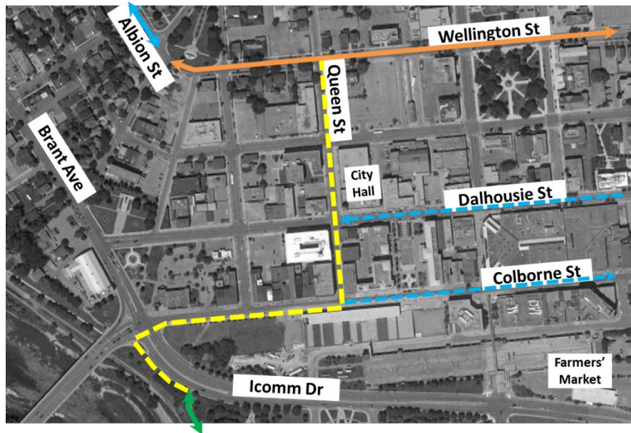
Figure 16: Design Concept at Brant Ave/ Colborne St/ Icomm Dr
