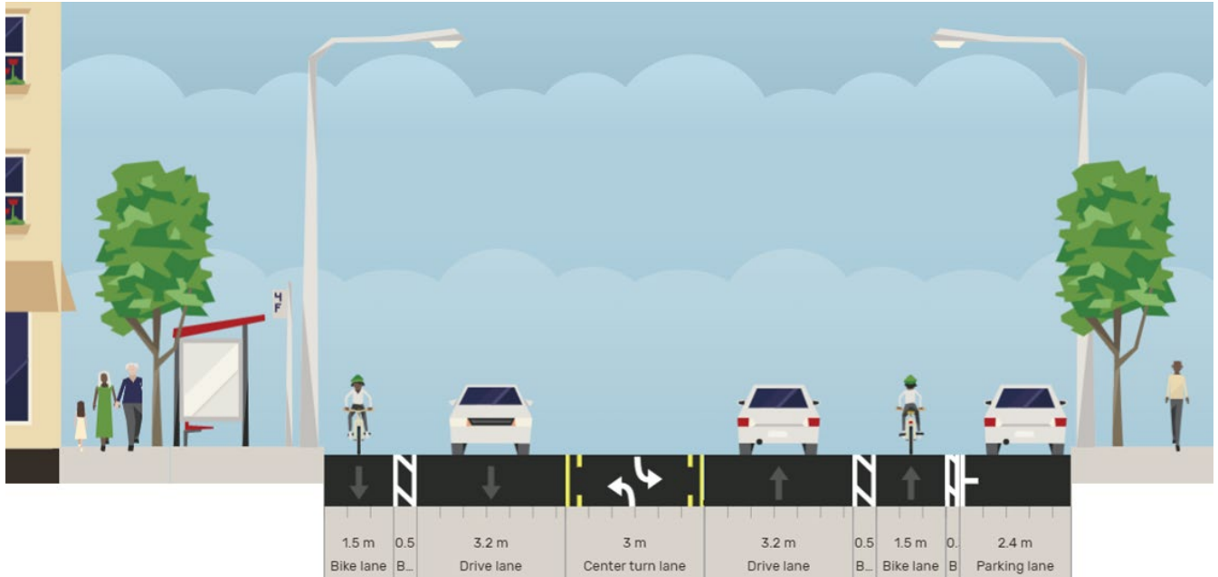
Figure 23: A Graphic Representation of the Sample Cross-section Described Above and in Appendix H
